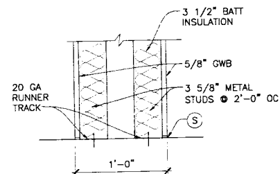
PARTITION 2 NON-LOAD BEARING
