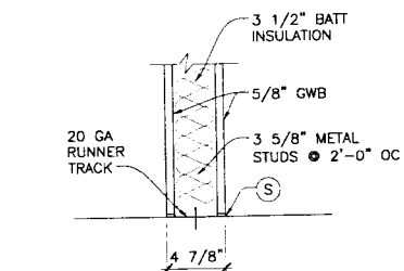
PARTITION 1 NON-LOAD BEARING 1 HOUR FIRE RATED ASSEMBLY
