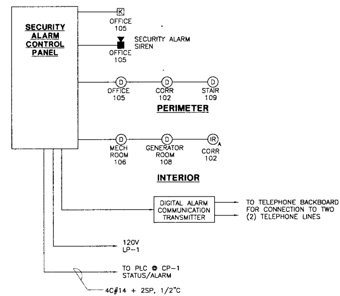
SECURITY SYSTEM RISER DIAGRAM NTS
