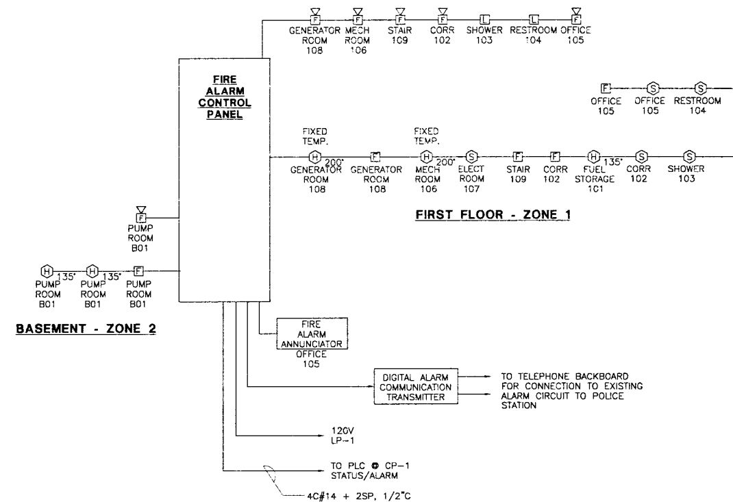
FIRE ALARM SYSTEM RISER DIAGRAM NTS
