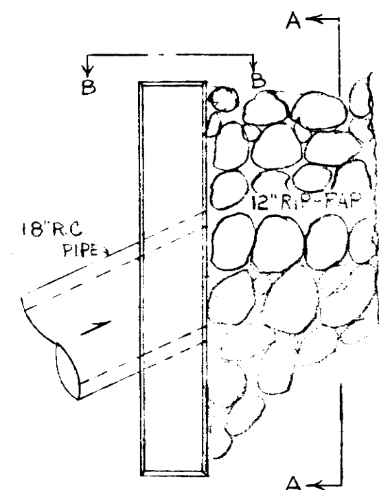
PLAN OF HEAD-WALL SCALE \frac{1}{2}''=1'-0''
