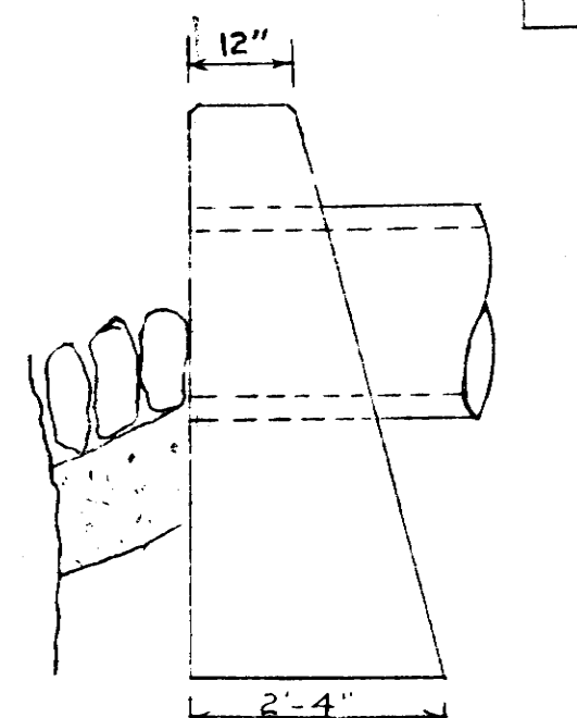
SECTION B-B SCALE \frac{1}{2}''=1'-0''
