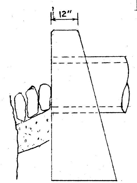
SECTION B-B SCALE 1/2"=1'-0"
