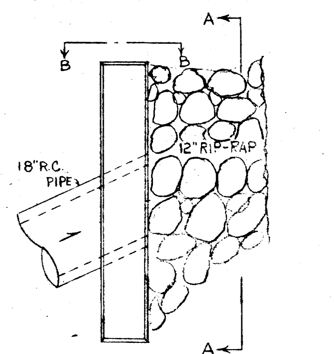
PLAN OF HEAD-WALL SCALE 1/2"=1'-0"
