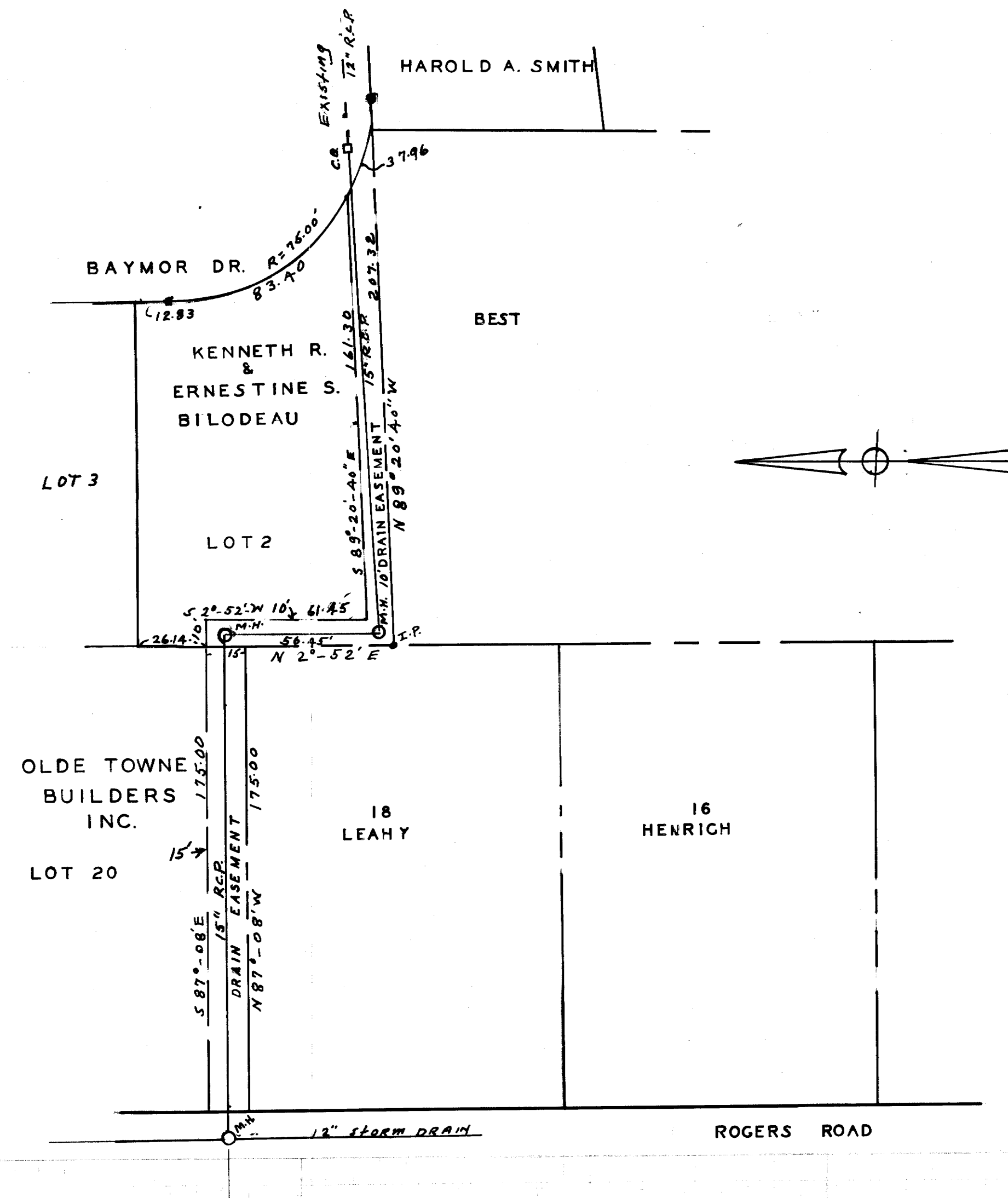
PLAN & PROFILE STORM DRAIN EASEMENT ROGERS RD. TO BAYMOR DR. SCALE 1"=40' HOR. 1"=4' VERT.
