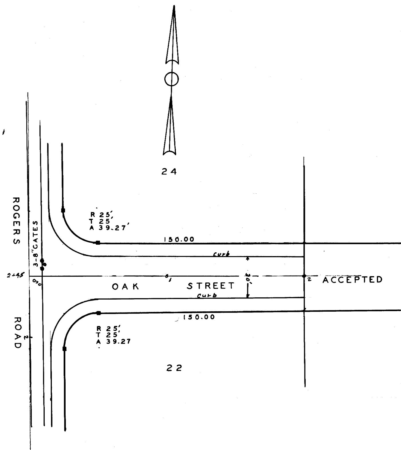
PLAN & PROFILE OAK STREET SCALE 1"=40' HOR. 1"=4' VERT. DEC. 1963 ROBERT T. BITTERS REG. L. S.
