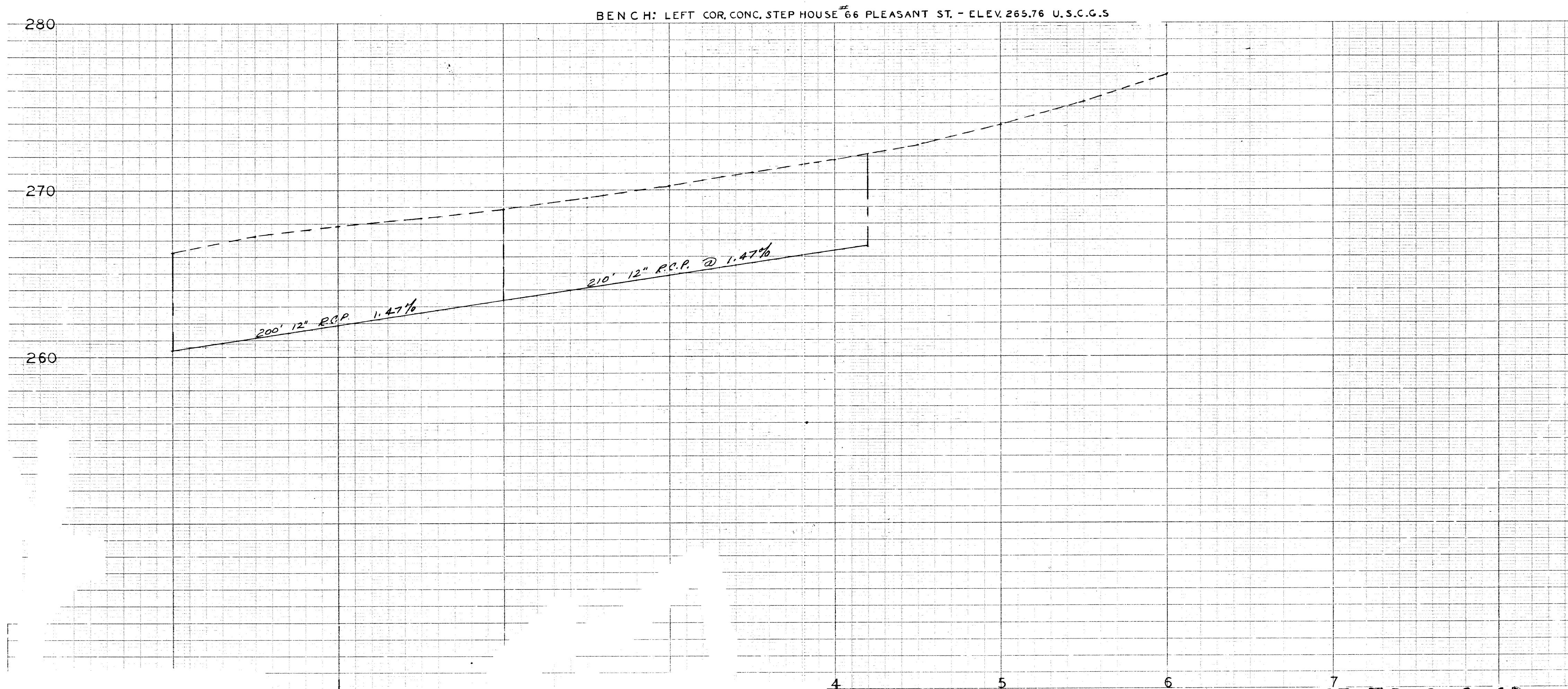
PLAN & PROFILE OF CALLENDER AVENUE DEPT. OF PUBLIC WORKS A. A. MELIEN, ENG. TOWN OF EAST LONGMEADOW MASSACHUSETTS SCALE: 1" = 40' HORIZ., 1" = 4' VERT APRIL, 1963
