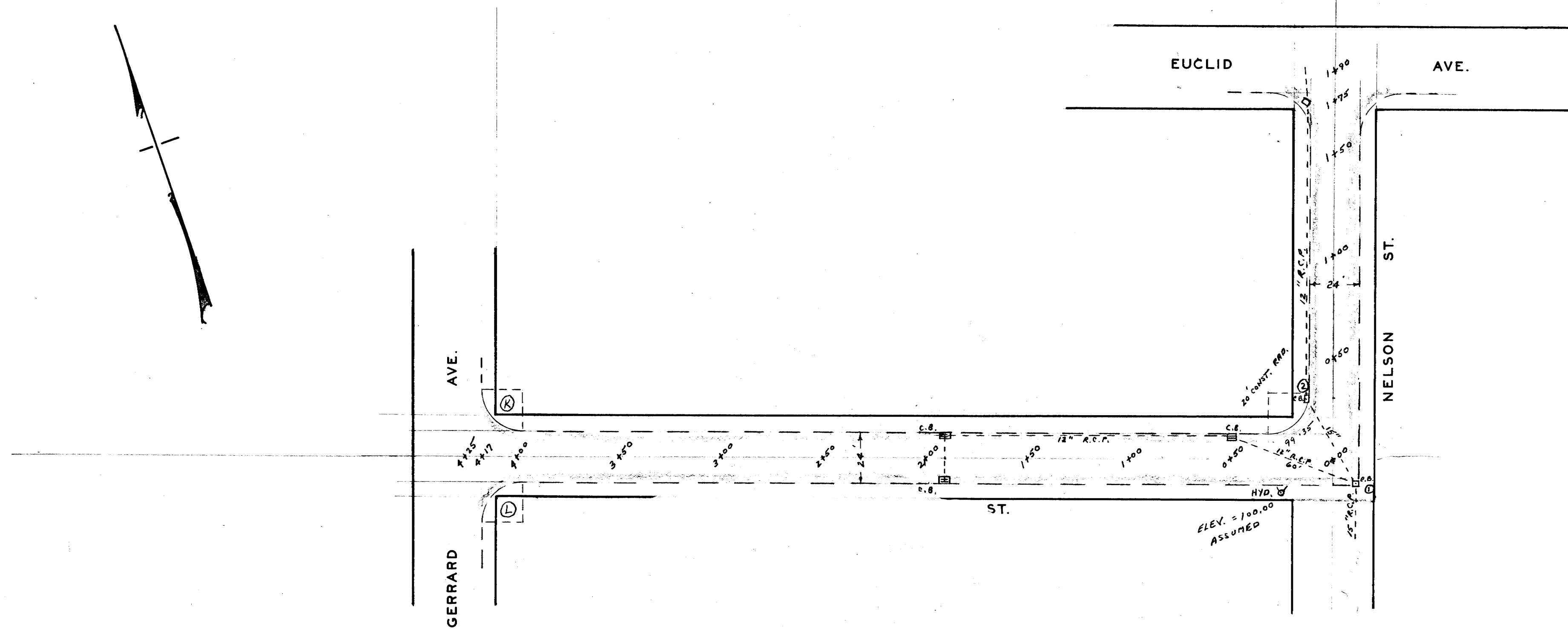
PLAN & PROFILE OF KELSEY & NELSON STREETS EAST LONGMEADOW MASS. SCALE: 1" = 40' HOR. 1" = 4' VERT. AUG. 1970 A. A. MELIEN TOWN ENG'R.
