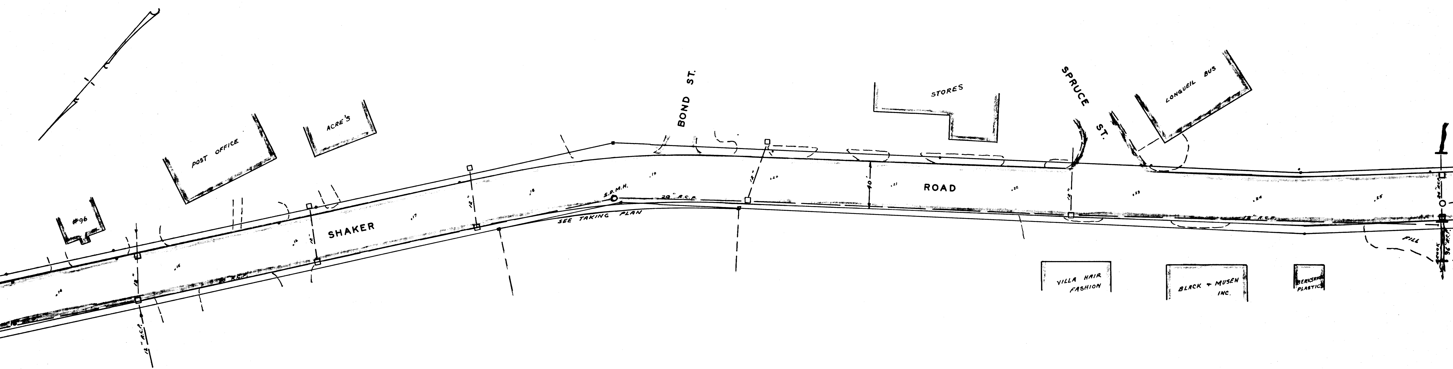
PLAN & PROFILE SHAKER ROAD EAST LONGMEADOW MASS. SCALE: 1" = 40' HOR. 1" = 4' VERT. JAN. 1973 A.A. MELIEN TOWN ENGR.
