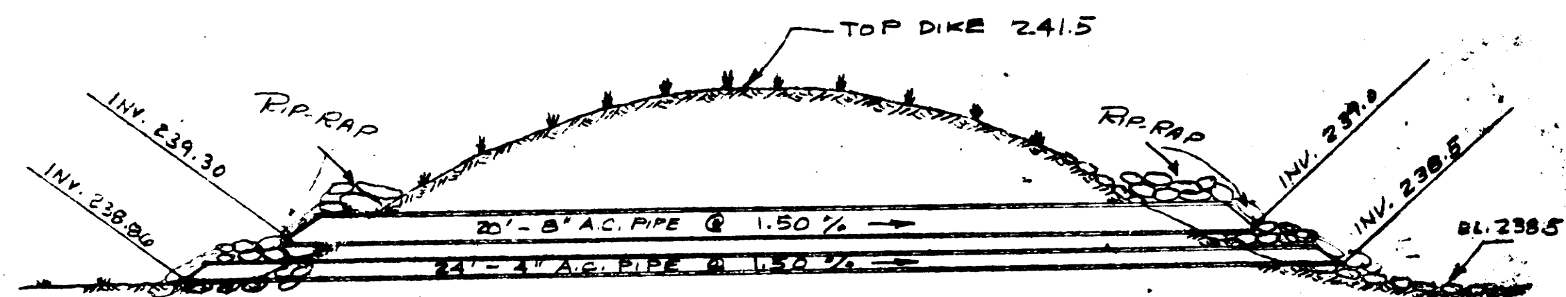
SECTION AT OUTLET PIPES
