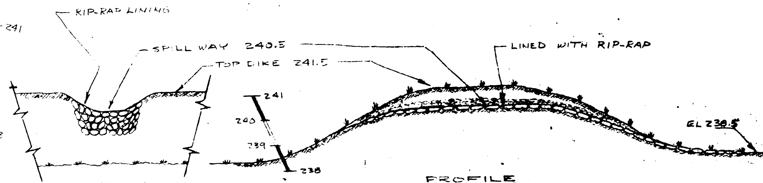
SECTION AT SPILLWAY
