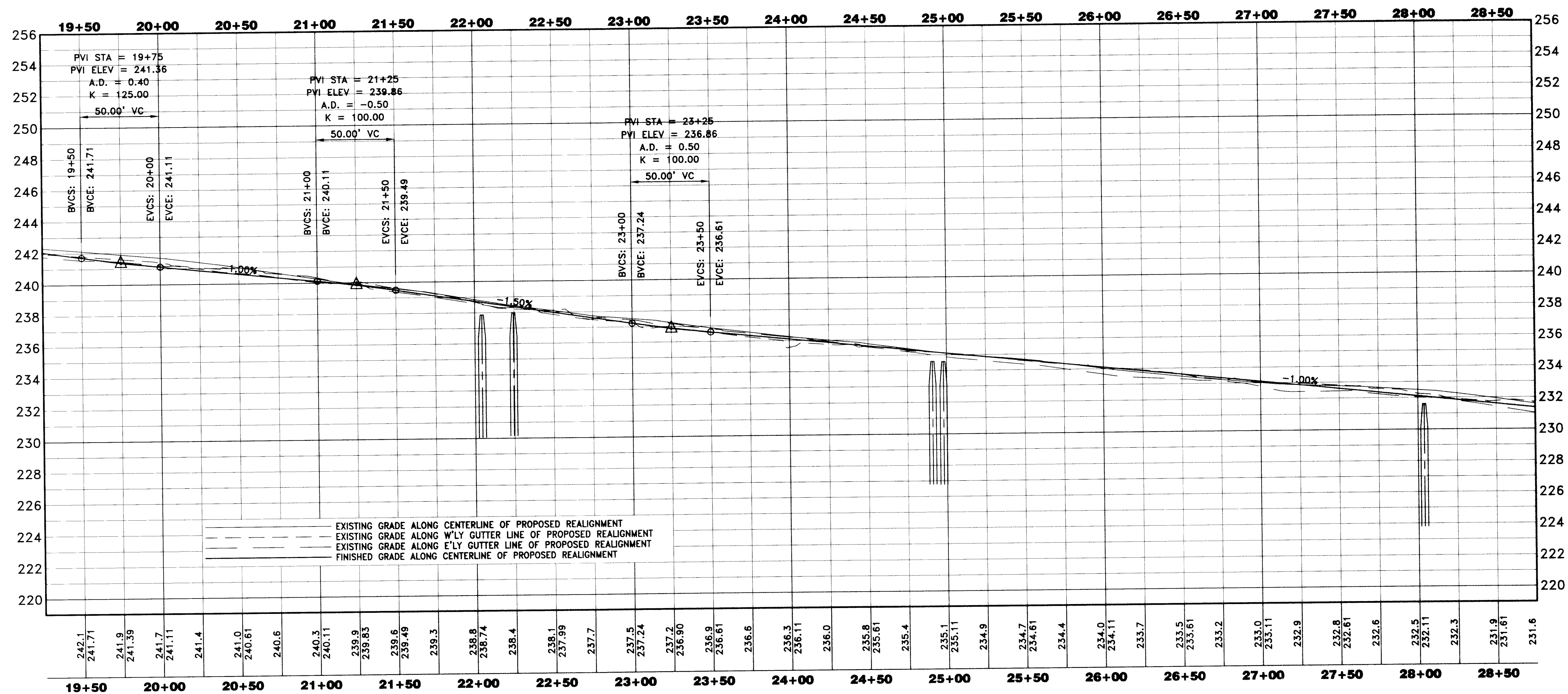
PROFILE SCALES HORIZONTAL 1"=40' VERTICAL 1"=4'
