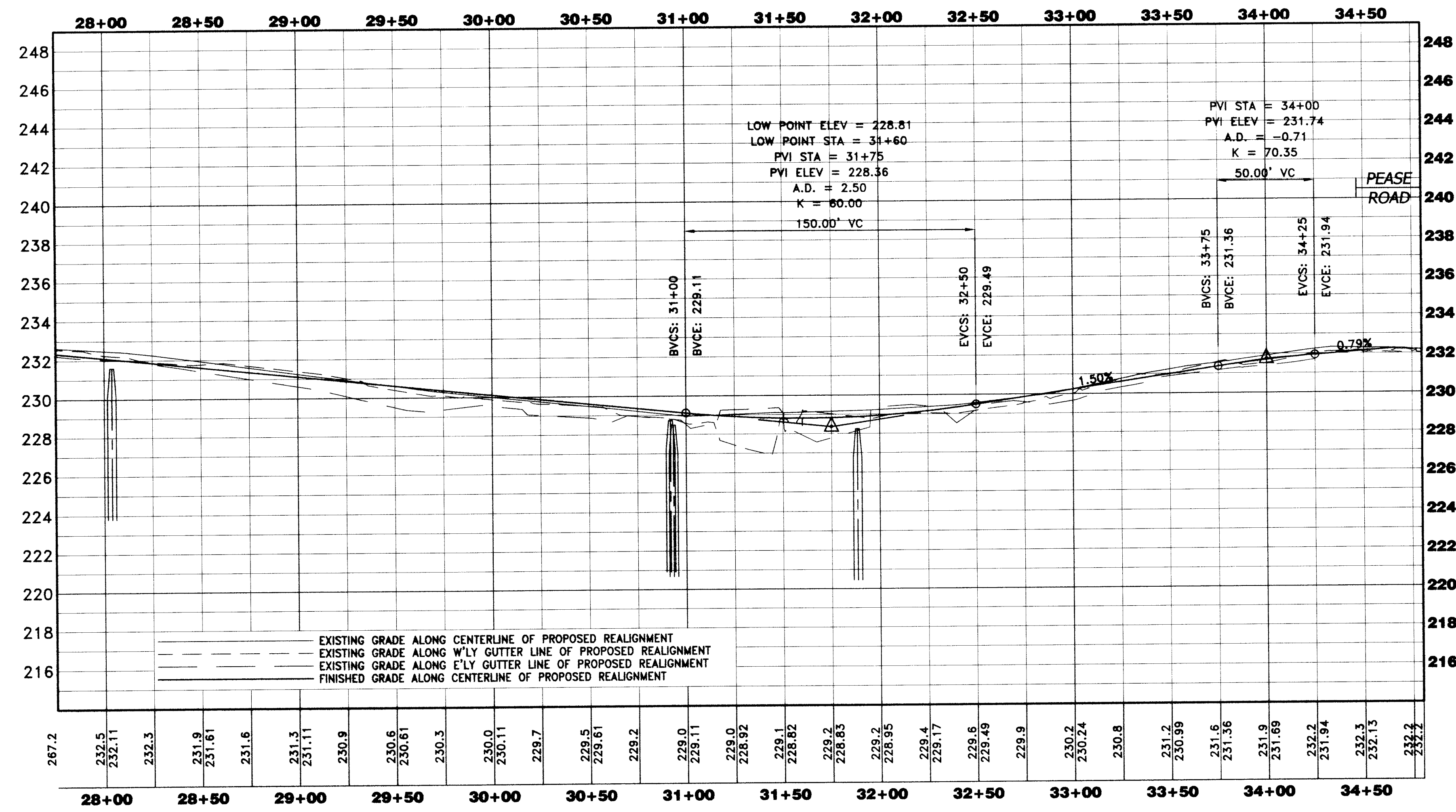
PROFILE SCALES HORIZONTAL 1"=40' VERTICAL 1"=4'
